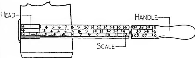
FIG. 45. LUMBERMAN'S BOARD STICK.
